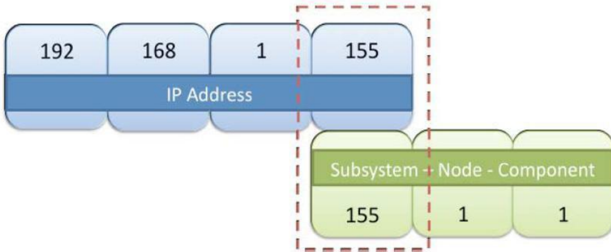
IP and JAUS ID Assignment
