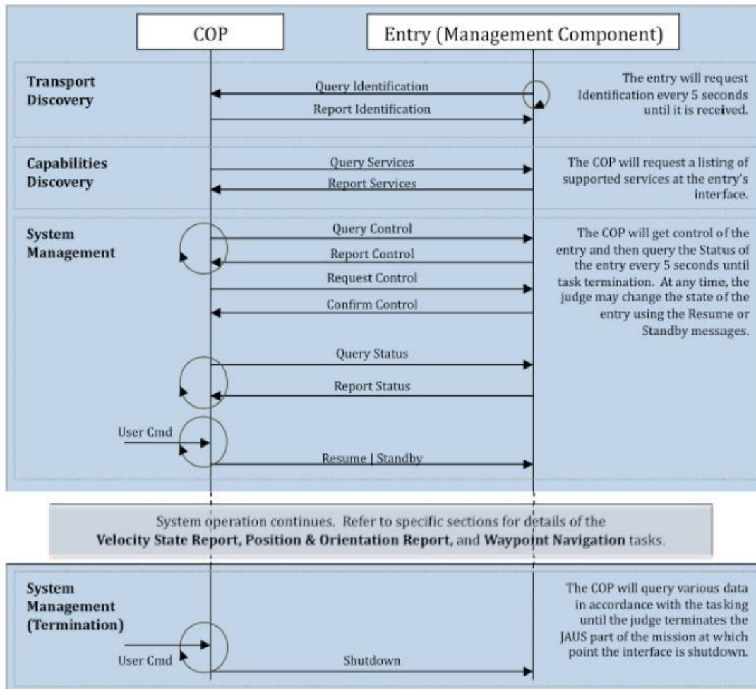
Discovery and System Management
