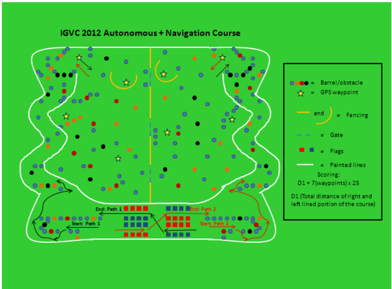
Example Auto-Nav Challenge Layout
