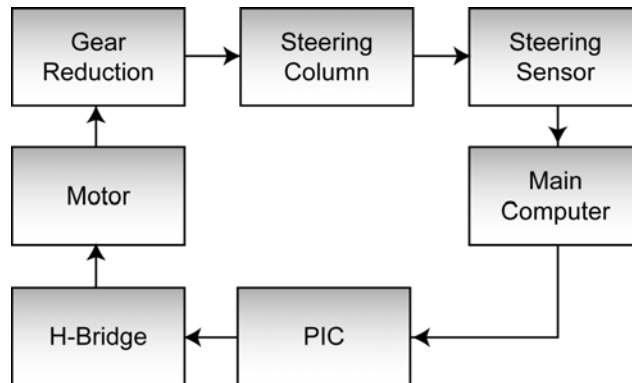
Figure 2 – Steering System
