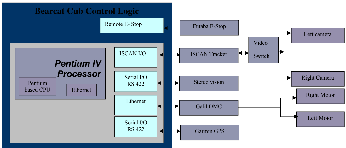
Figure 5. Bearcat Cub block diagram
