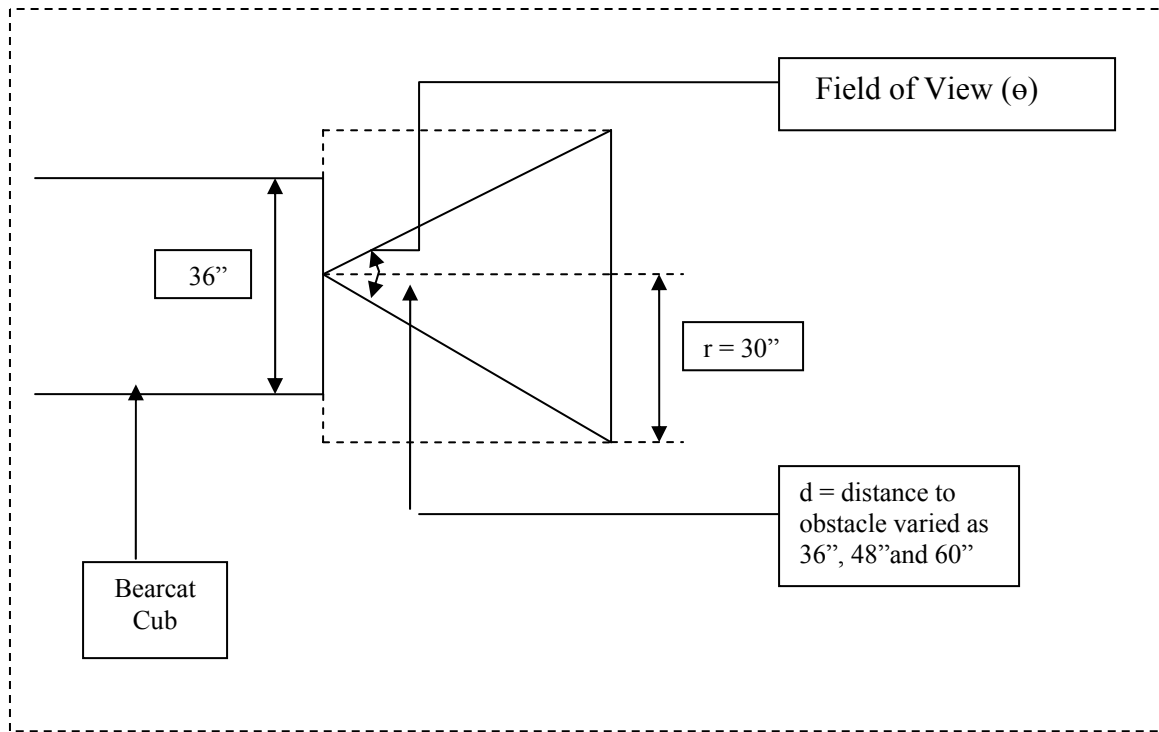
Figure 7. Stereo vision system
